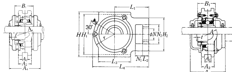
Cast dust cover type Open end C-UKT...D1 Closed end CM-UKT...D1
