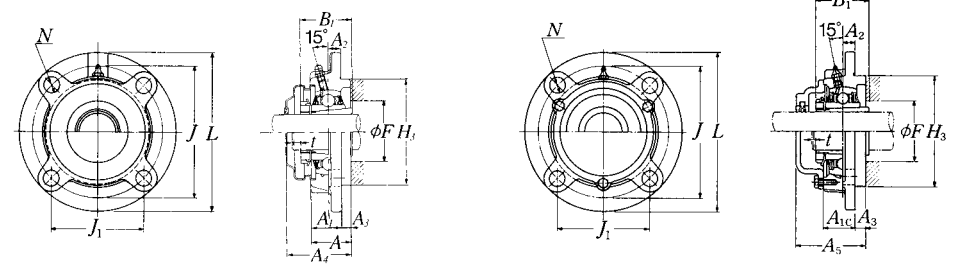
Pressed steel dust cover type Open end Z-UKFC...D1 Closed end ZM-UKFC...D1
