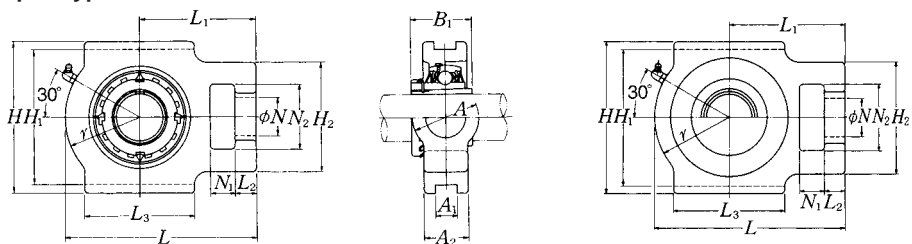
Pressed steel dust cover type Open end Z-UKT...D1 Closed end ZM-UKT...D1
