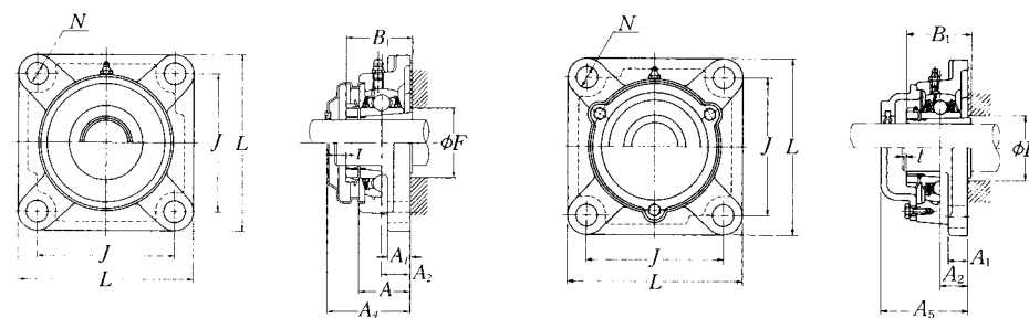
Pressed steel dust cover type
