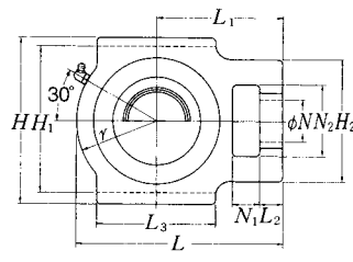
Pressed steel dust cover type Open end Z-UCT...D1 Closed end ZM-UCT...D1
