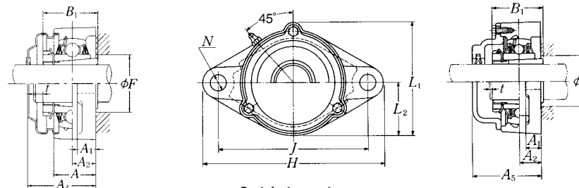
Cast dust cover type Open end C-UKFL...D1 Closed end CM-UKFL...D1
