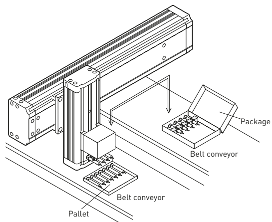
6 - Work feed in stamping machine
