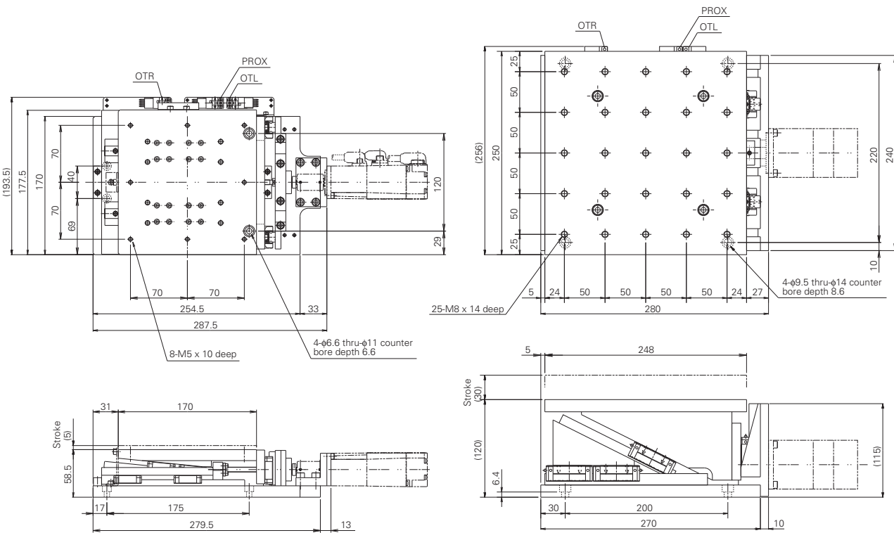
XY-HW0001-34D * (Reduction ratio 1/10)
