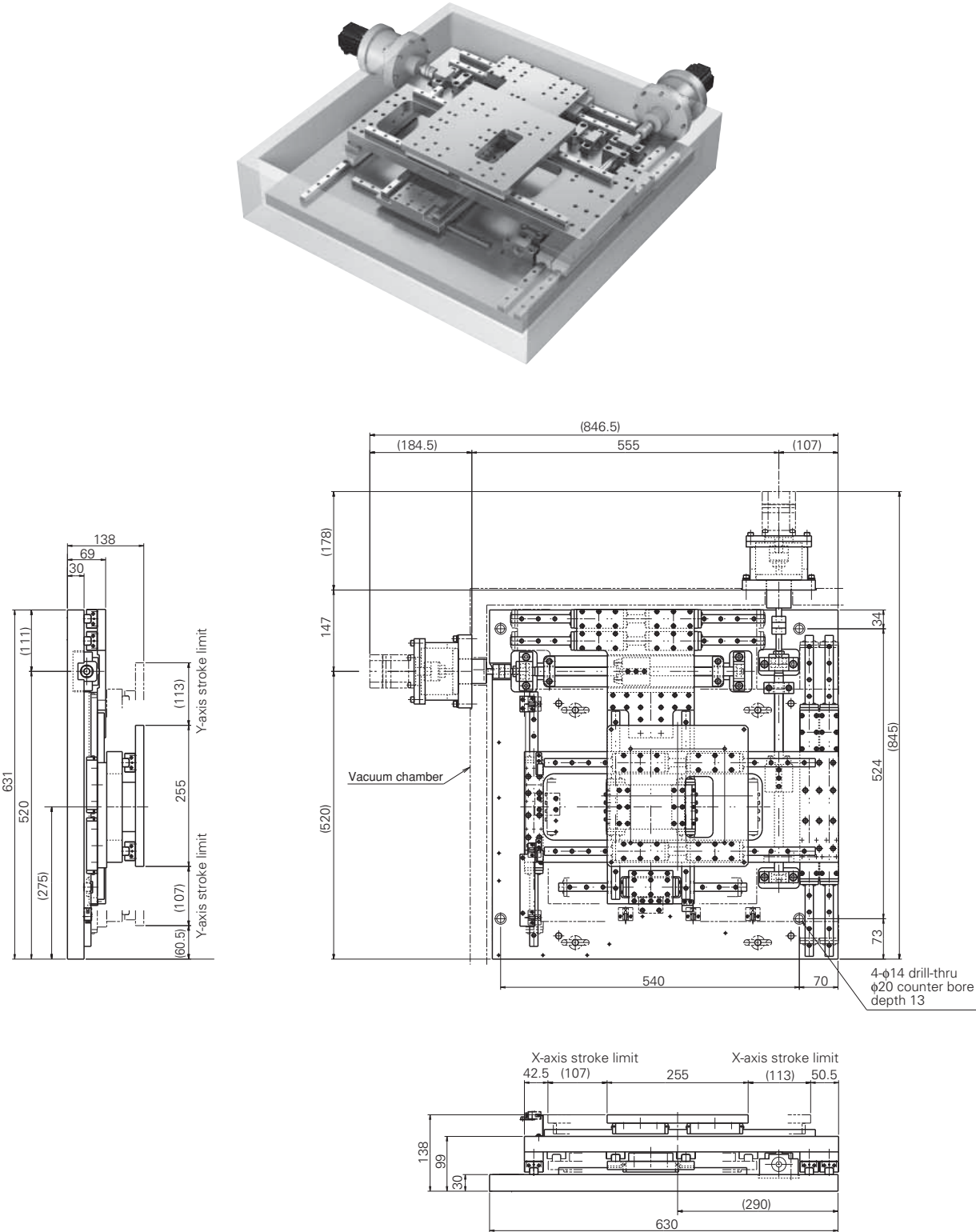
(2) HT series: Example (8 inches)
