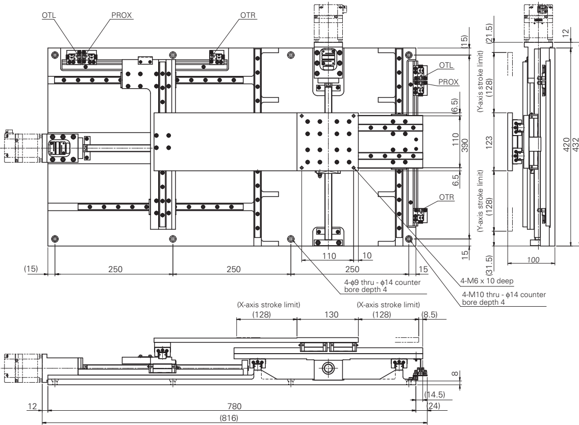
XY-HT2525-34*(Stroke 250 mm x 250 mm type)
