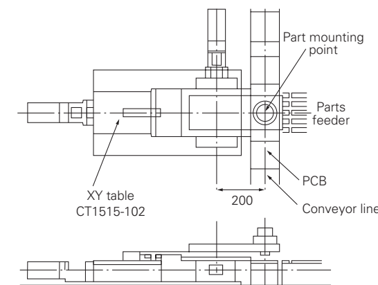
Schematic of XY Table Application as Chip Mouter Fig. (7)-1
