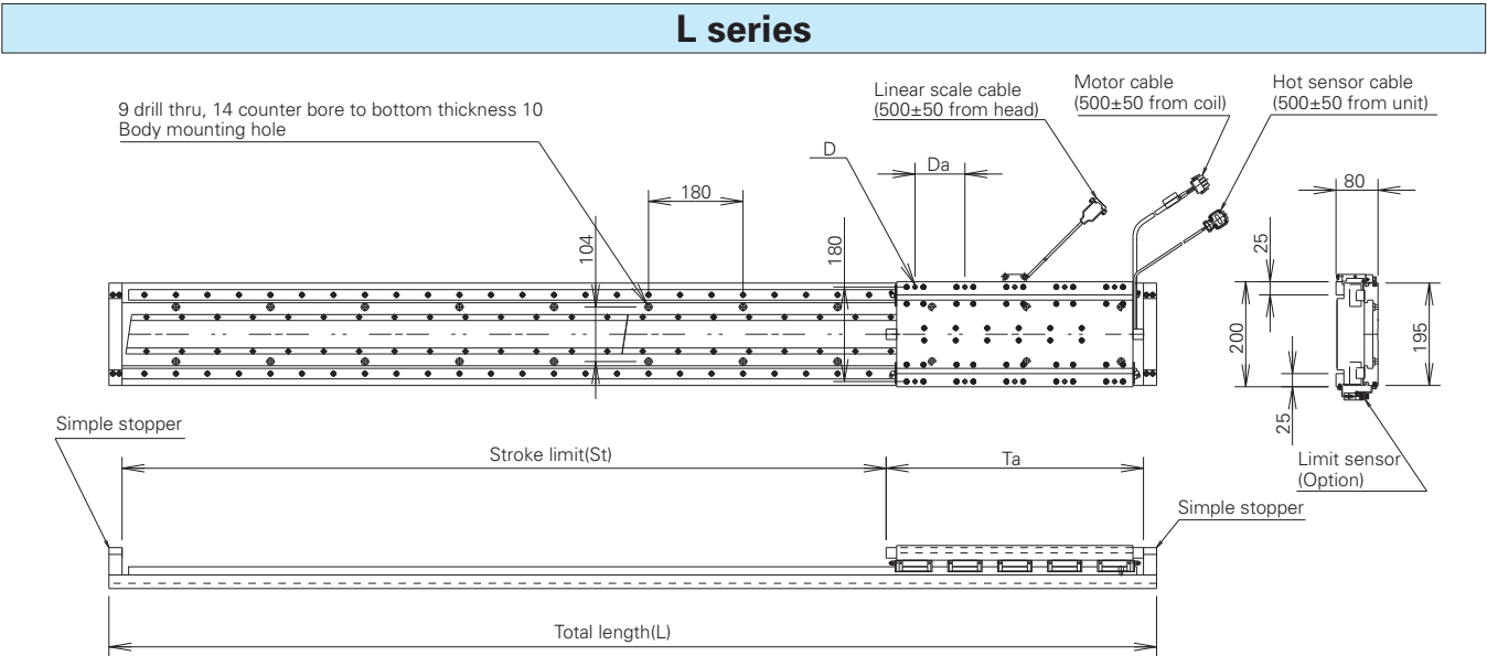
L series: Dimensions
