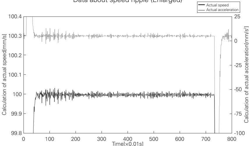
Data about speed ripple (Enlarged)
