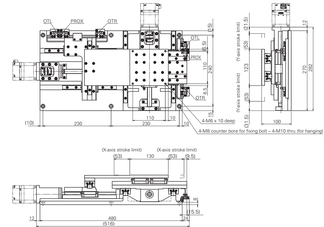
XY-HT1010-34*(Stroke 100 mm x 100 mm type)
