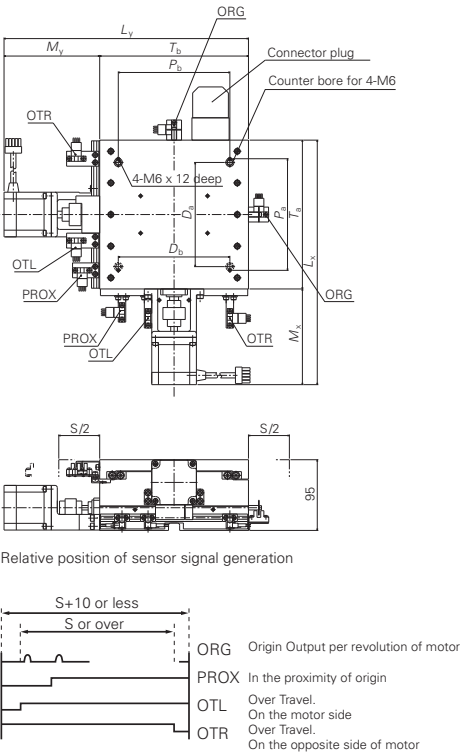
CD type two-axis table (Compact)
