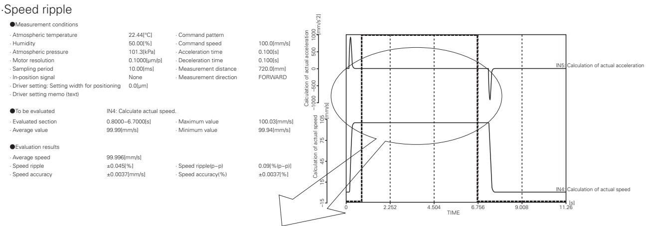
Data about speed ripple (Enlarged)
