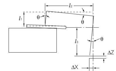
Relation between Positioning Table and Working Point Fig. (7)-2
