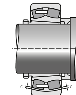
Fig. 4 Measuring clearance in large spherical roller bearing
