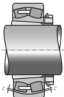
Fig. 3 Clearance measurement of spherical roller bearing
