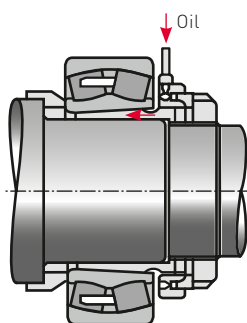
Fig. 2 Mounting with hydraulic nut
