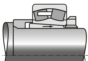
Fig. 1 Mounting with adapter
