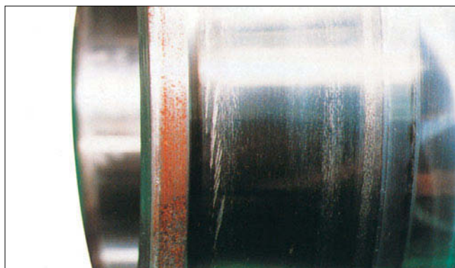
Part: Inner ring of a spherical roller bearing Symptom: Partial smearing occurs circumferentially on raceway surface Cause: Incorrect lubrication
