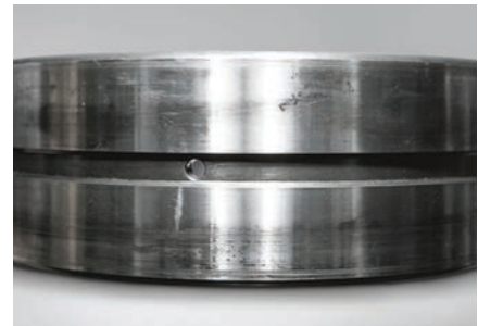
Part: Outer ring of a spherical roller bearing Observation: Creep occurs over entire circumference of outside surface Cause: Loose fit between outer ring and housing
