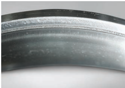
Part: Inner ring of a spherical roller bearing
