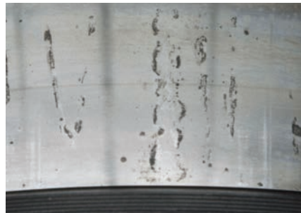
Part: Inner ring of a spherical roller bearing Observation: Rust on raceway surface at roller pitch Cause: Entry of water into lubricant
