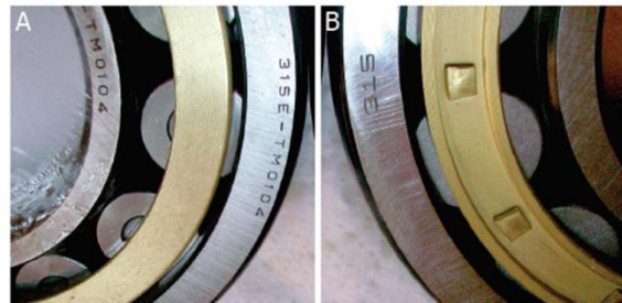
A. Authentic NSK product B. Counterfeit
