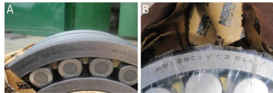
A. Authentic NSK product B. Counterfeit
